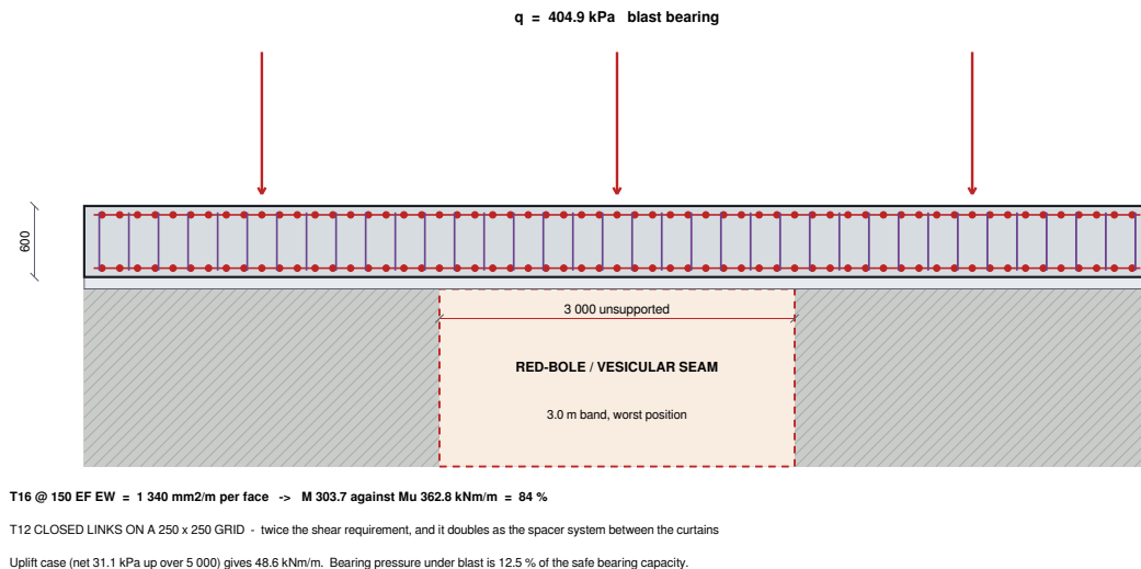
Fig 7.3 : Mat Foundation, Governing Soft-Band Case
