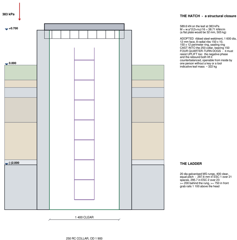
Fig 8.2 : Escape Shaft Head, Hatch and Ladder
