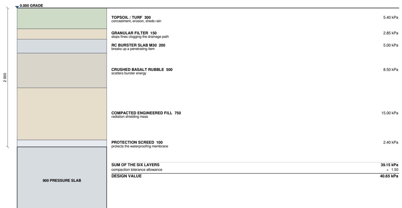
THE ENGINEERED COVER - 2 000 mm IN SIX LAYERS
