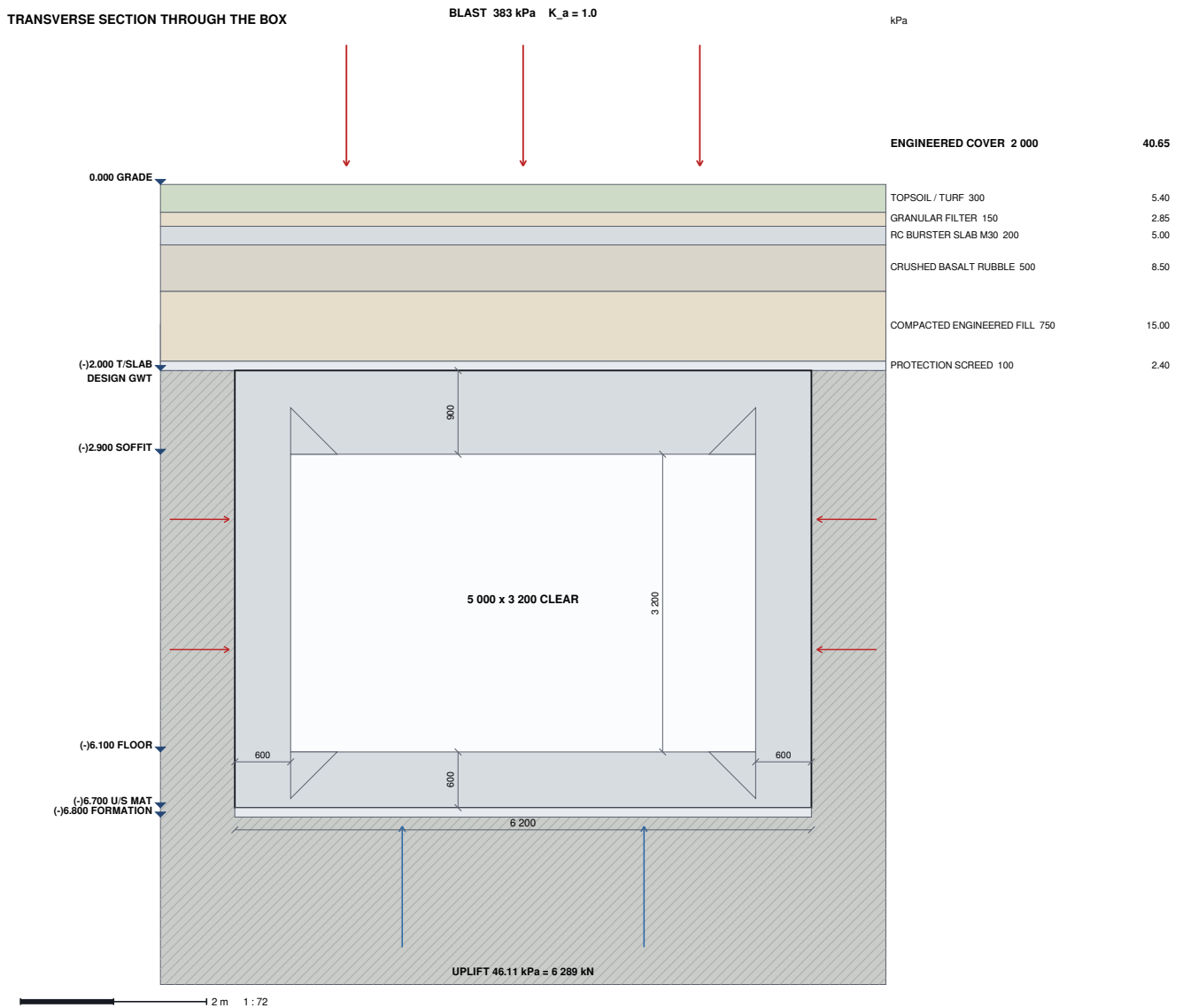
Fig 3.3 : Transverse Section through the Box
