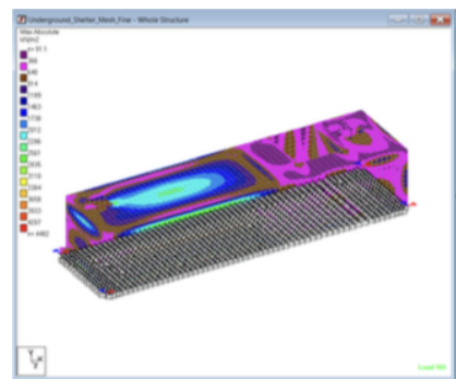
(f) Fine mesh, plate stress
