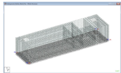
(c) Fine mesh, 4 552 plates
