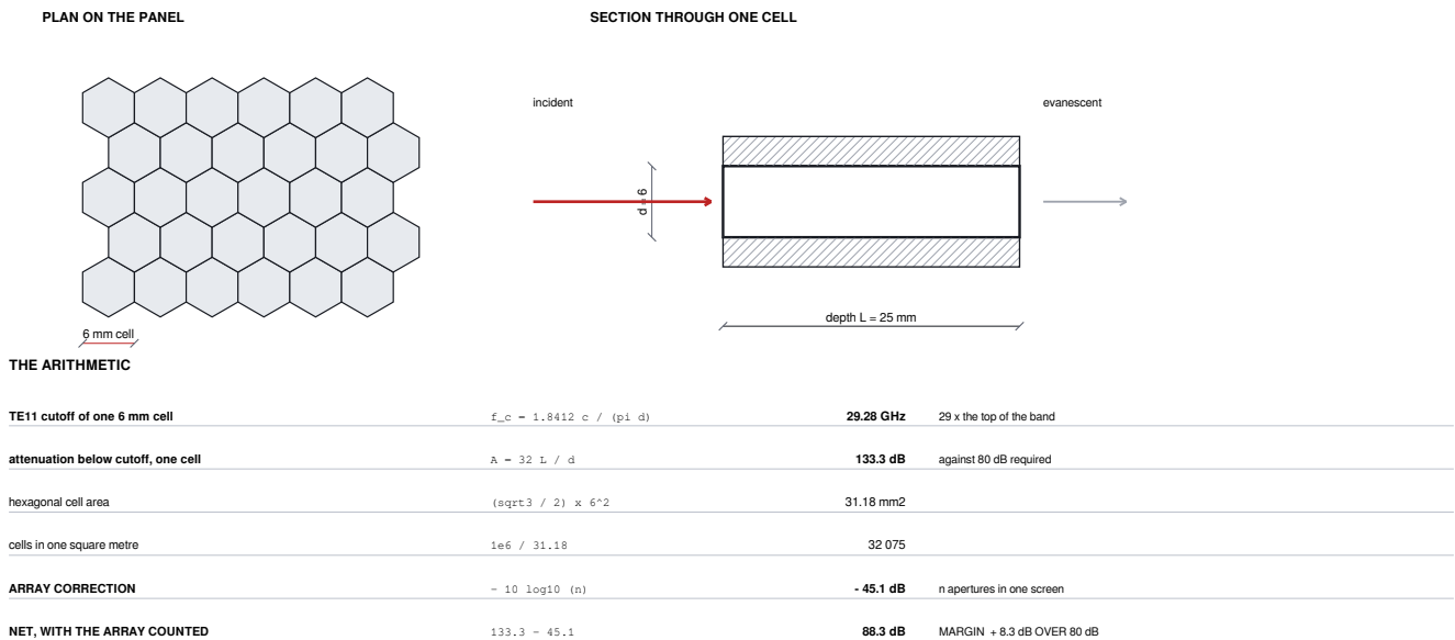
Fig 11.3 : Honeycomb Waveguide Ventilation Panel
