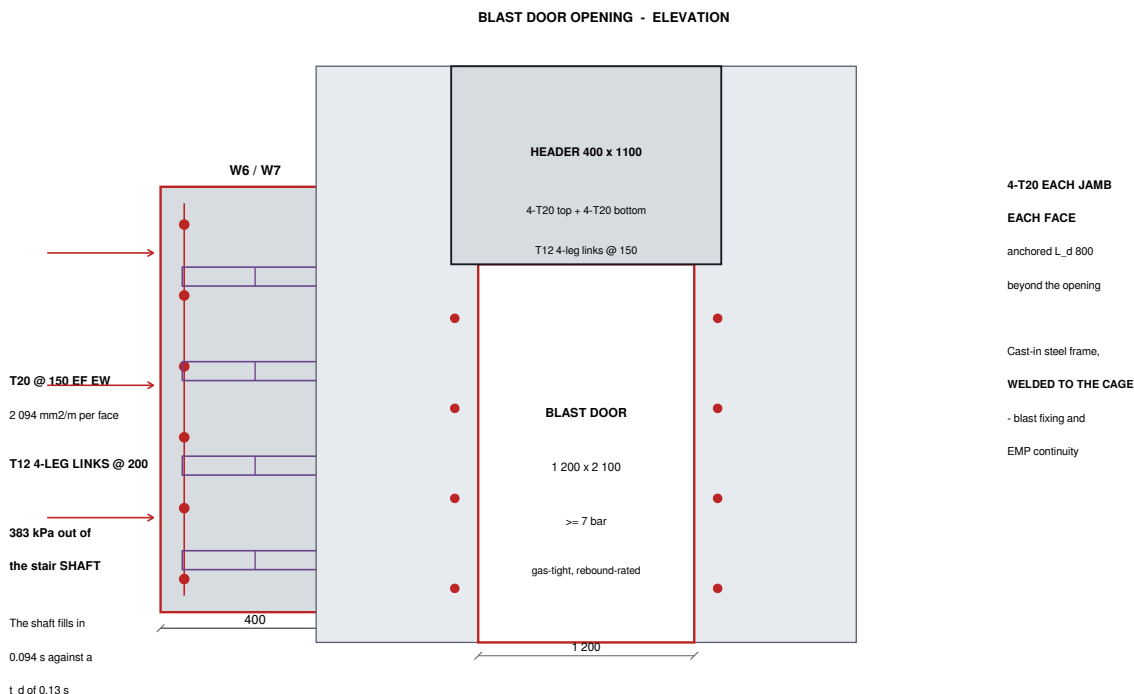
Fig 7.2 : Walls W6 and W7 with the Blast Door Opening
