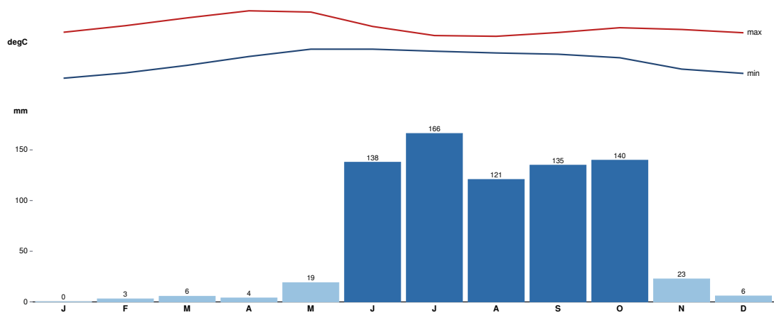
Fig 2.8 : Monthly Rainfall and Temperature at the Site
