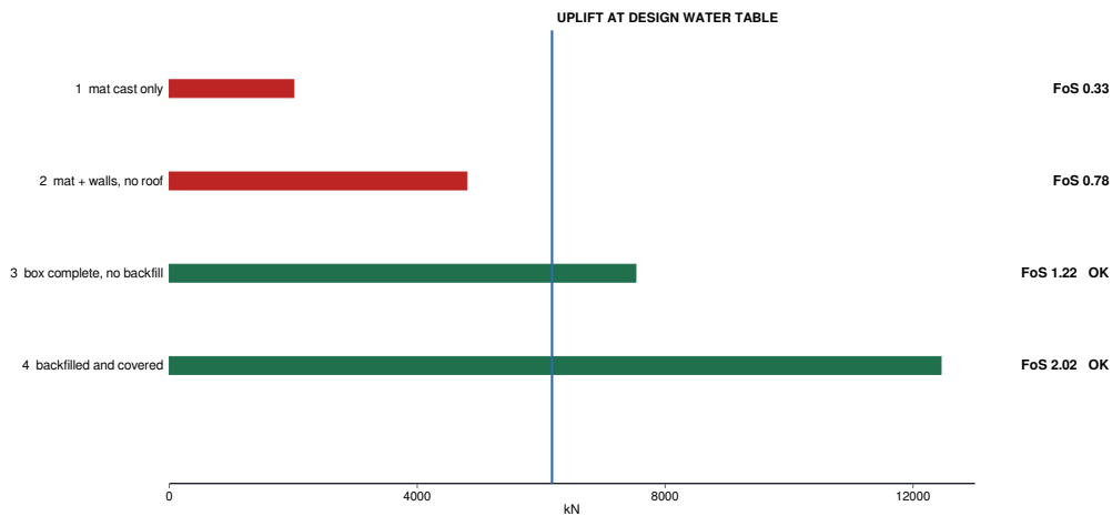
FLOTATION CHECK AT EACH CONSTRUCTION STAGE
