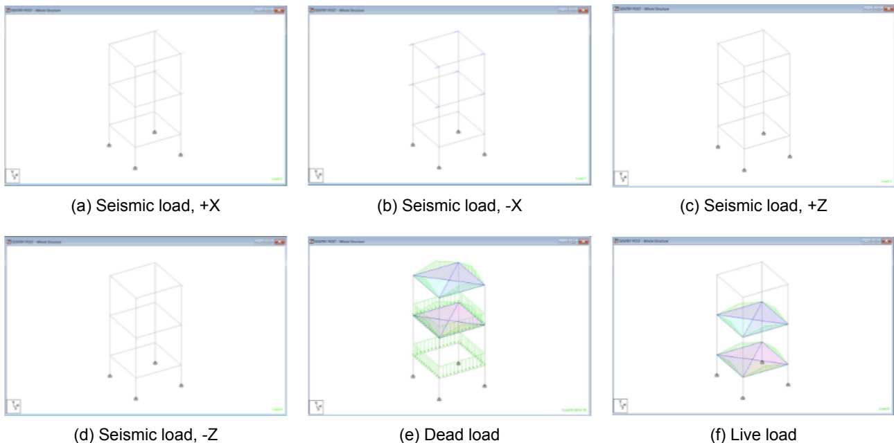
Fig 6.6 : Load Cases, Sentry Post Frame Model (STAAD.Pro)
